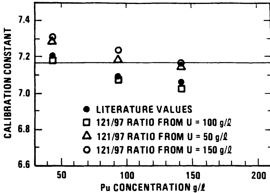
Fig. 4. A plot of the calibration constant \Delta\mu d in \text{cm}^3/\text{g} vs plutonium concentration. Each point represents a different correction factor \alpha determined by the ratio between the 121- and 97-keV transmitted peaks for each uranium solution or by literature values.
