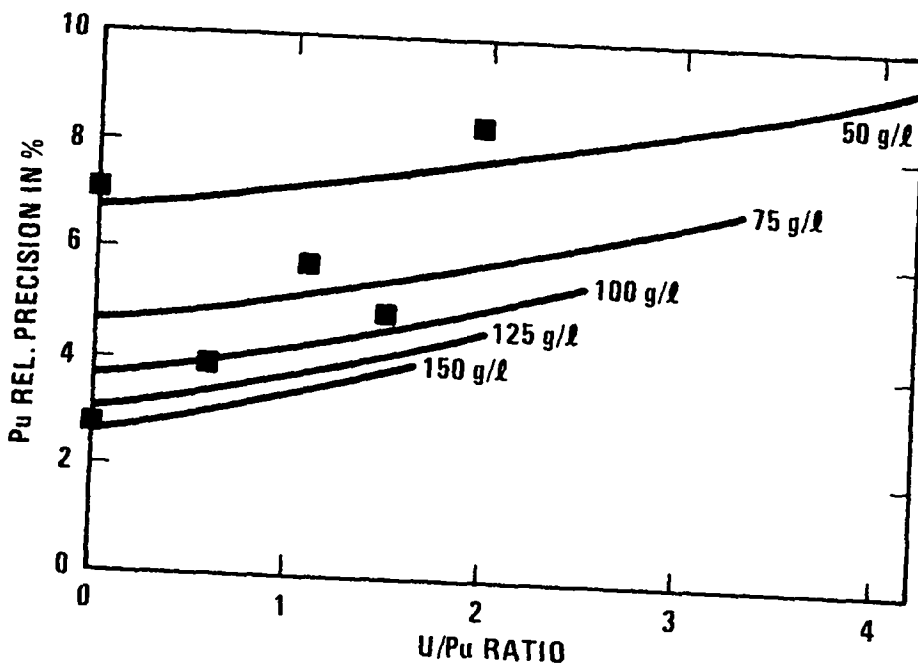
Fig. 7. A plot of expected per cent precision ( 1\sigma ) vs the U/Pu ratio for a 2000-s counting time and different plutonium concentrations. The blocks represent the measured precision.
