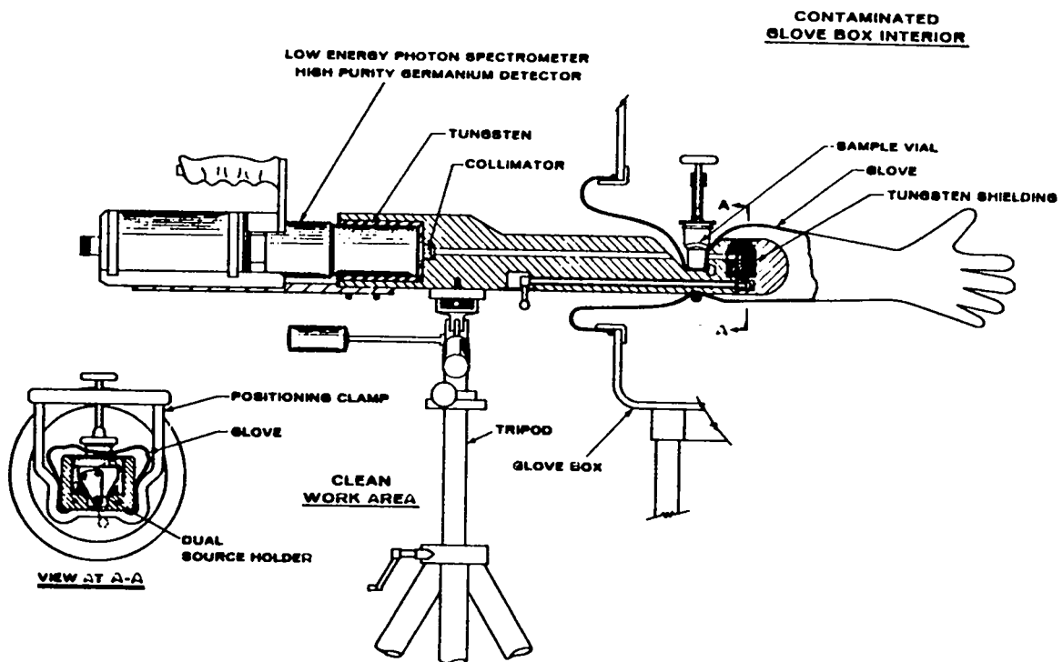
Fig. 2. Measuring head of the compact K-edge densitometer used for testing the performance of the TEGA technique.
