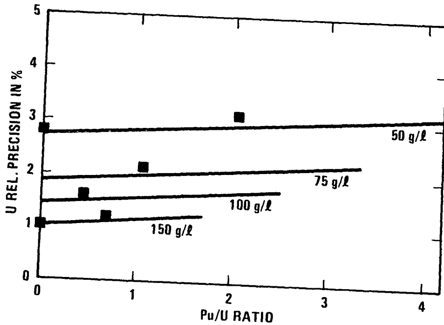
Fig. 6. A plot of expected per cent precision ( 1\sigma ) vs Pu/U ratio for a 2000-s counting time and different uranium concentrations. The blocks represent the measured precision.
