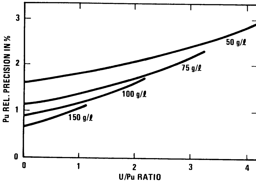
Fig. 8. A plot of the expected relative precision in plutonium assay vs U/Pu ratio for 1000-s counting time and different plutonium concentrations. The ^{75}\text{Se} source activity was assumed to be 100 mCi; that of the distance source detector, 14 cm.
