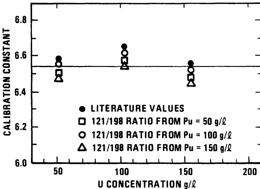
Fig. 5. The same plot as in Fig. 4, but vs uranium concentration. The correction factor \beta was determined by the ratio between the 121- and 198-keV transmitted peaks for each plutonium solution or by literature values.
