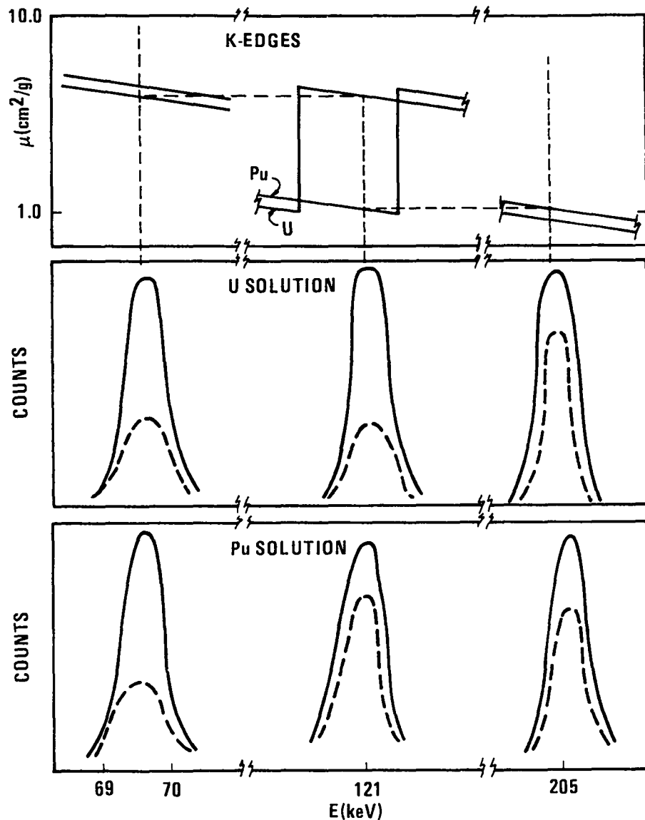
Fig. 1. Upper: an expanded view of the mass attenuation coefficient around the K-edge region vs gamma-ray energy for plutonium and uranium. Middle: a schematic representation of the transmitted photon intensities for "blank" (solid curves) and uranium-bearing solution (dotted curves). Lower: a schematic representation of the transmitted photon intensities for "blank" (solid curves) and plutonium-bearing (dotted curves) solution.
