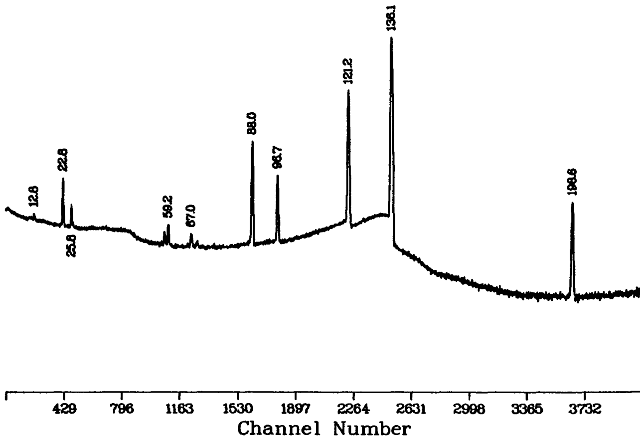
Fig. 3. Typical straight-through spectrum of transmission source. The 88-keV peak from a ^{109}\text{Cd} source can be used for counting loss correction.
